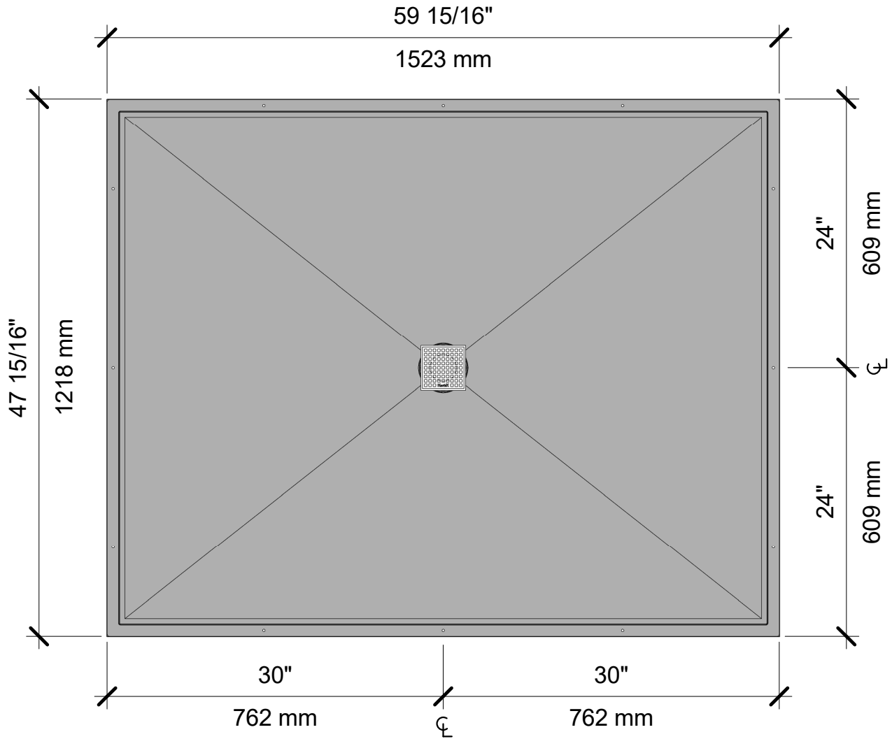
① KurbX STRUCTURAL SHOWER PAN - 60" X 48" 1" = 1'-0"
