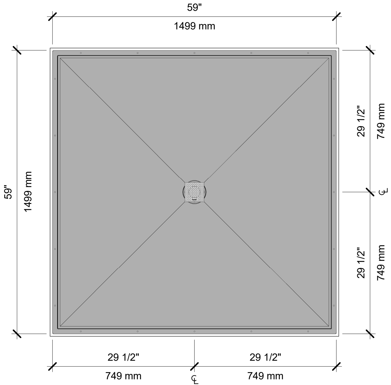
① KurbX STRUCTURAL SHOWER PAN - 59" X 59" 1" = 1'-0"
